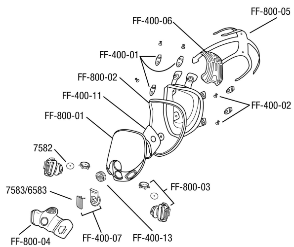
Figure 1: Despiece FF-800
